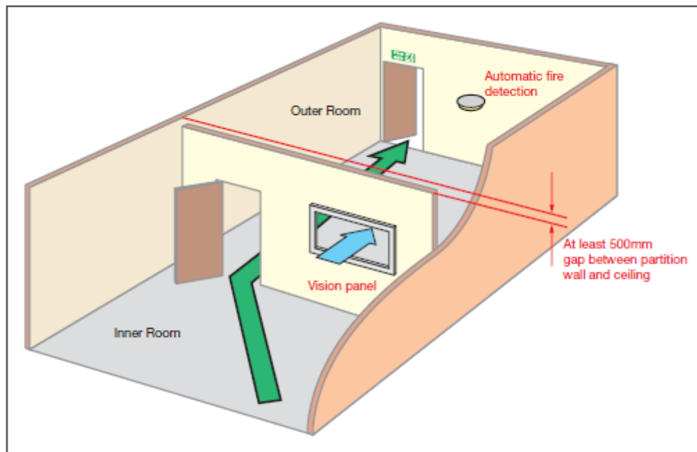
Figure 27: Inner rooms
