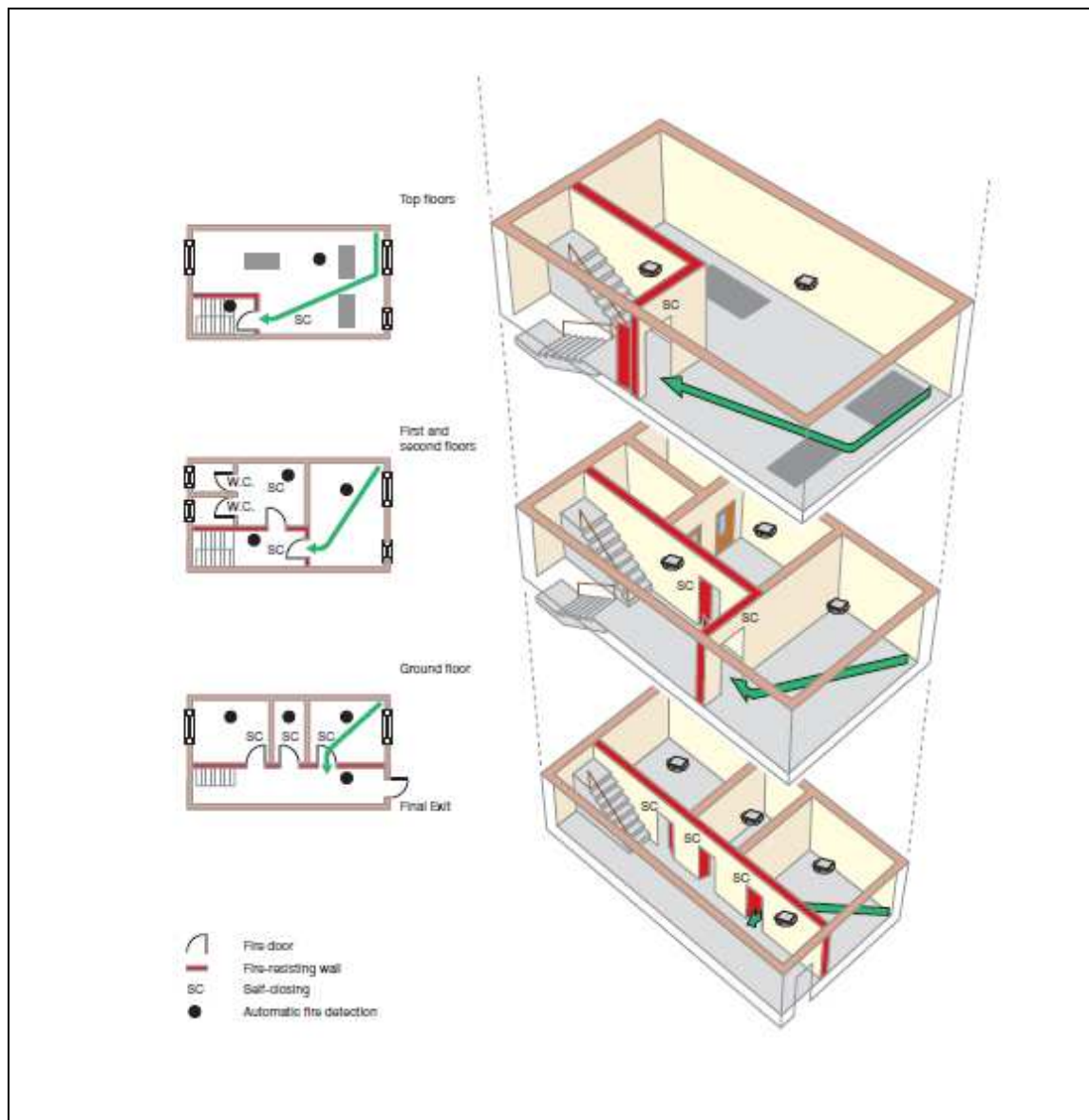
Figure 50: Ground and up to three upper storeys – protected with automatic fire detection (non-sleeping areas with very low risk)
