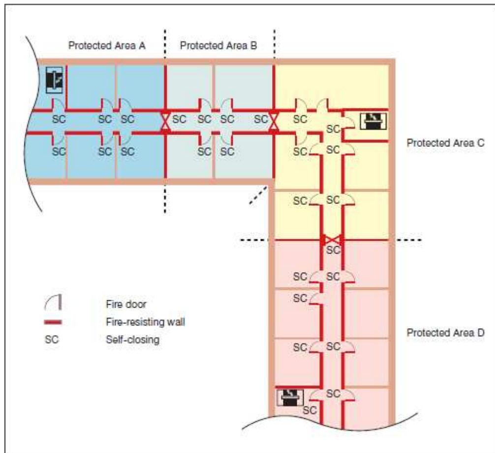
Figure 22: Protected areas in horizontal evacuation
