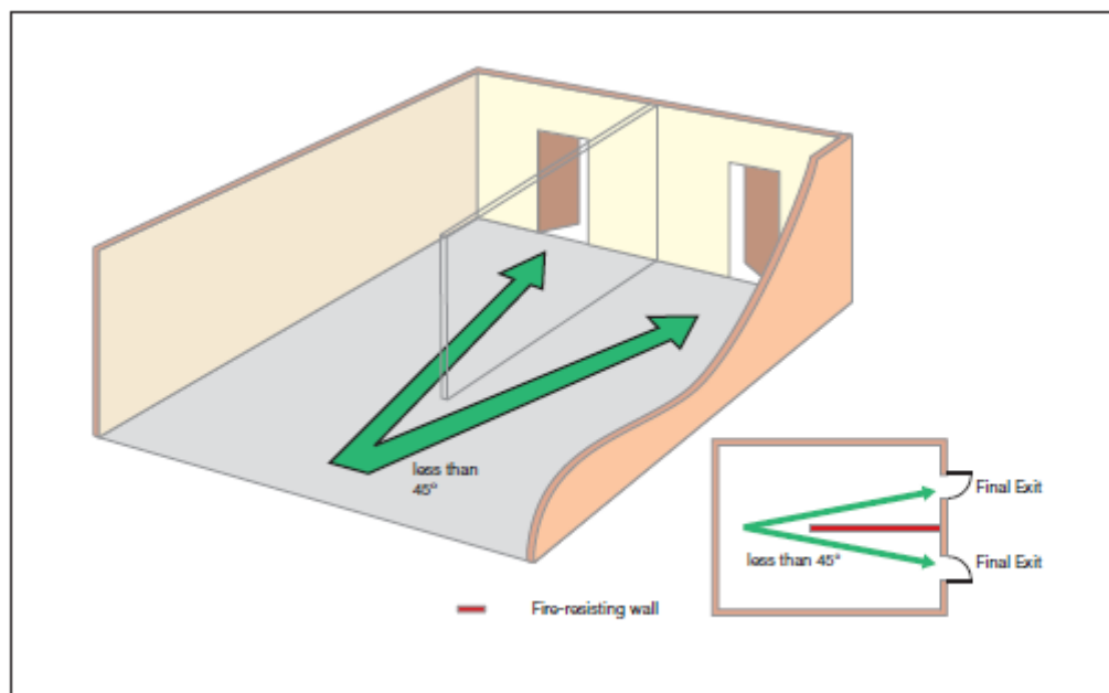
Figure 26: Alternative exits (separated by fire-resisting construction)
