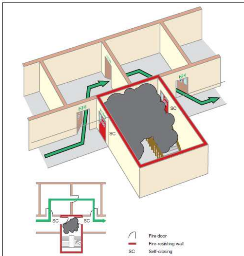
Figure 41: A stairway bypass route
