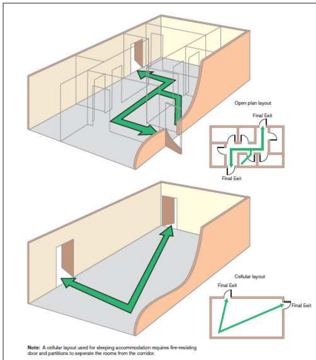
Figure 44: Ground floor with more than one exit (cellular and open plan)
