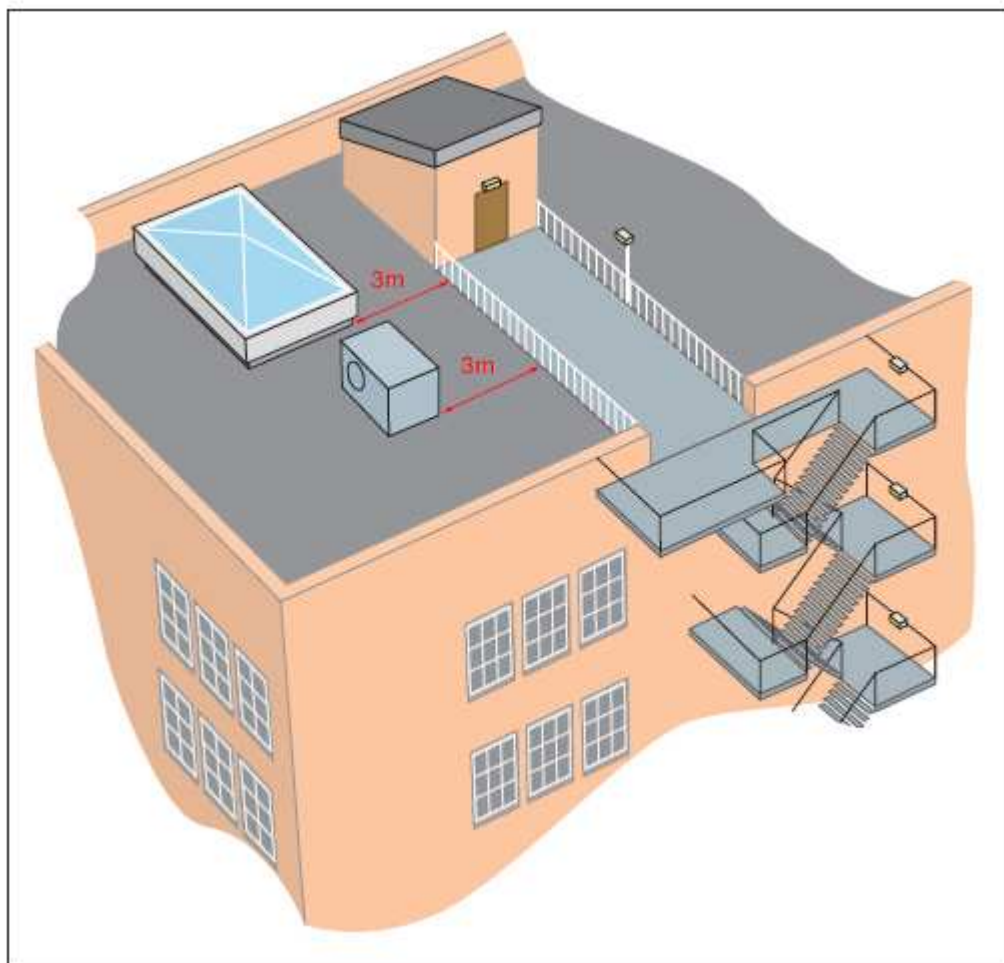
Figure 43: An escape route across a roof
