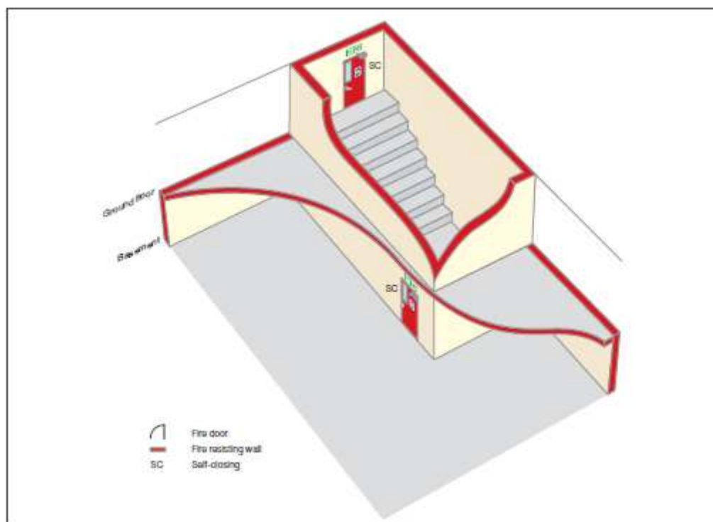
Figure 34: Basement protection
