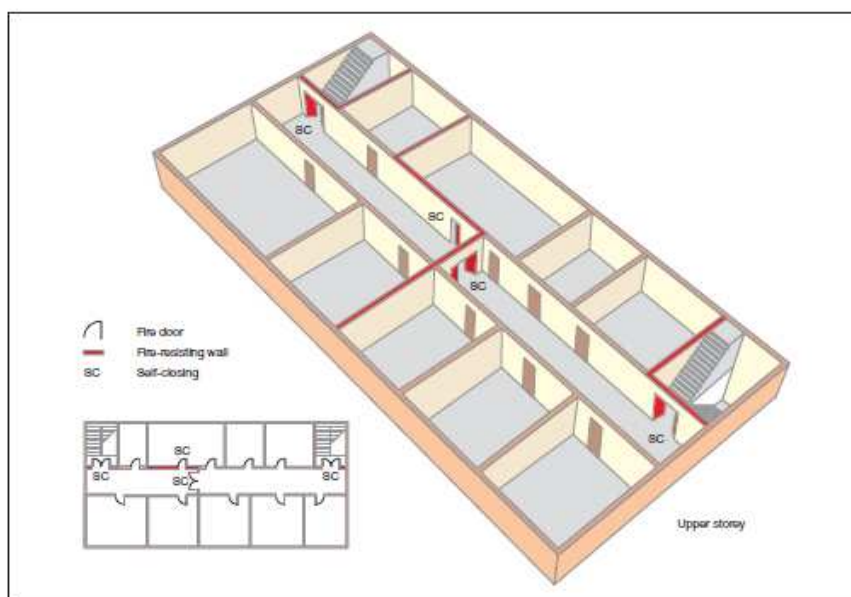
Figure 35: Subdivision of corridor between two stairways
