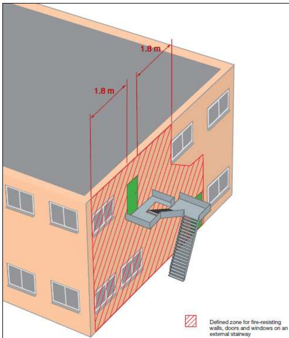
Figure 42: Protection to an external stairway
