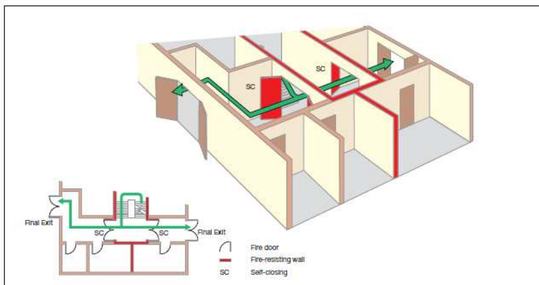
Figure 38: Examples of two escape routes from a stairway to final exits
