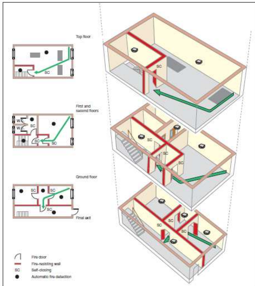
Figure 49: Ground and up to three upper storeys – protected by lobbies/corridors (sleeping areas)
