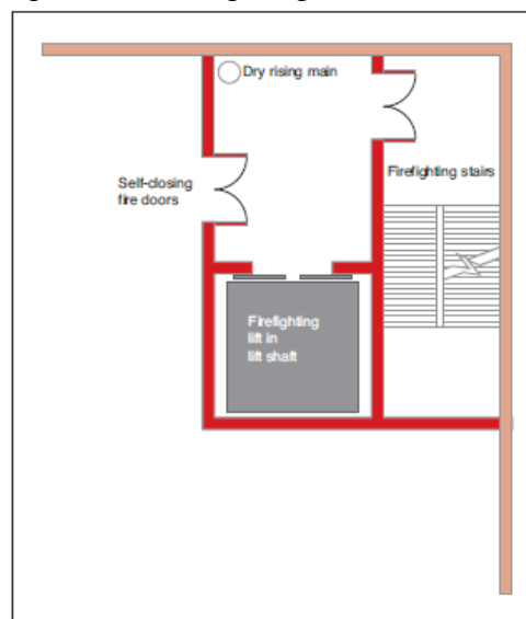
Figure 20: Firefighting shaft
