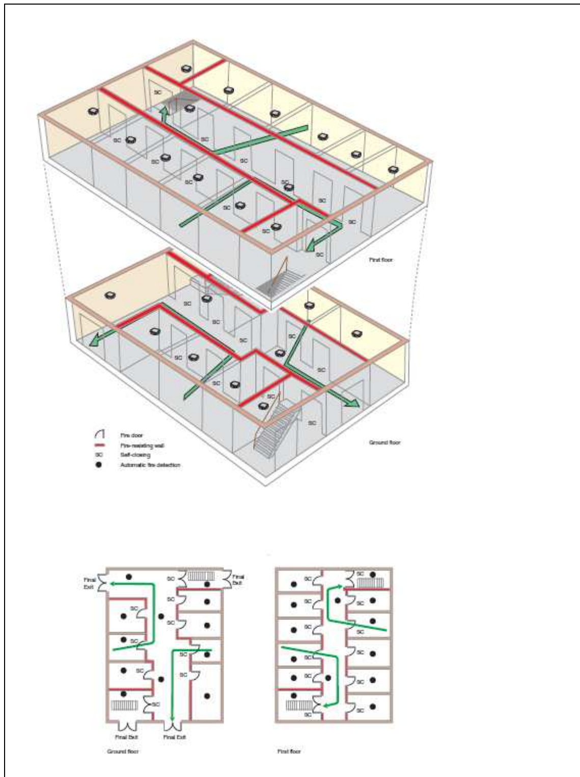
Figure 46: Two-storey with protected corridor (sleeping areas)
