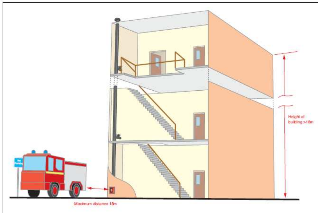
Figure 21: Rising main
