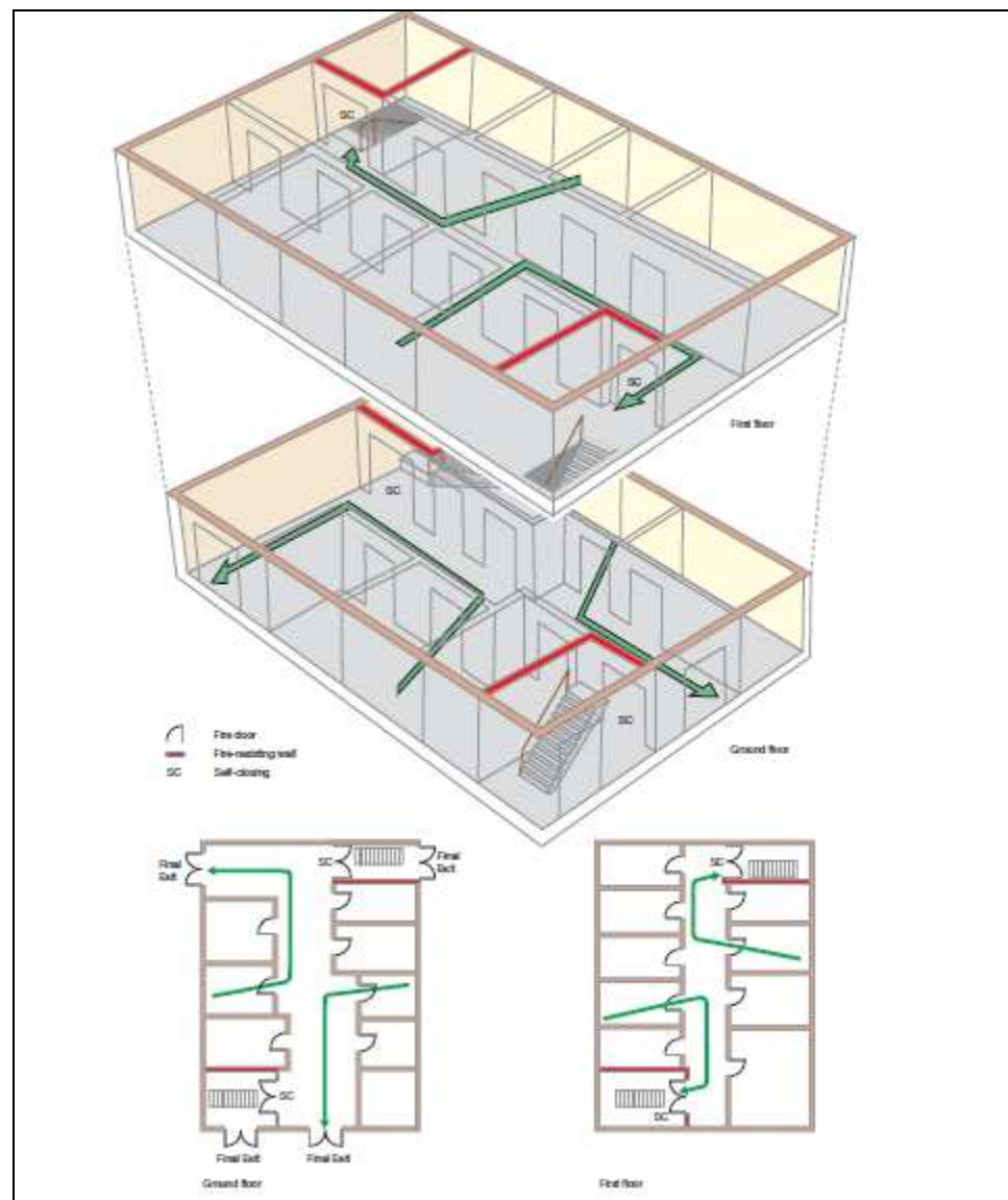
Figure 45: Two-storey (non sleeping areas)
