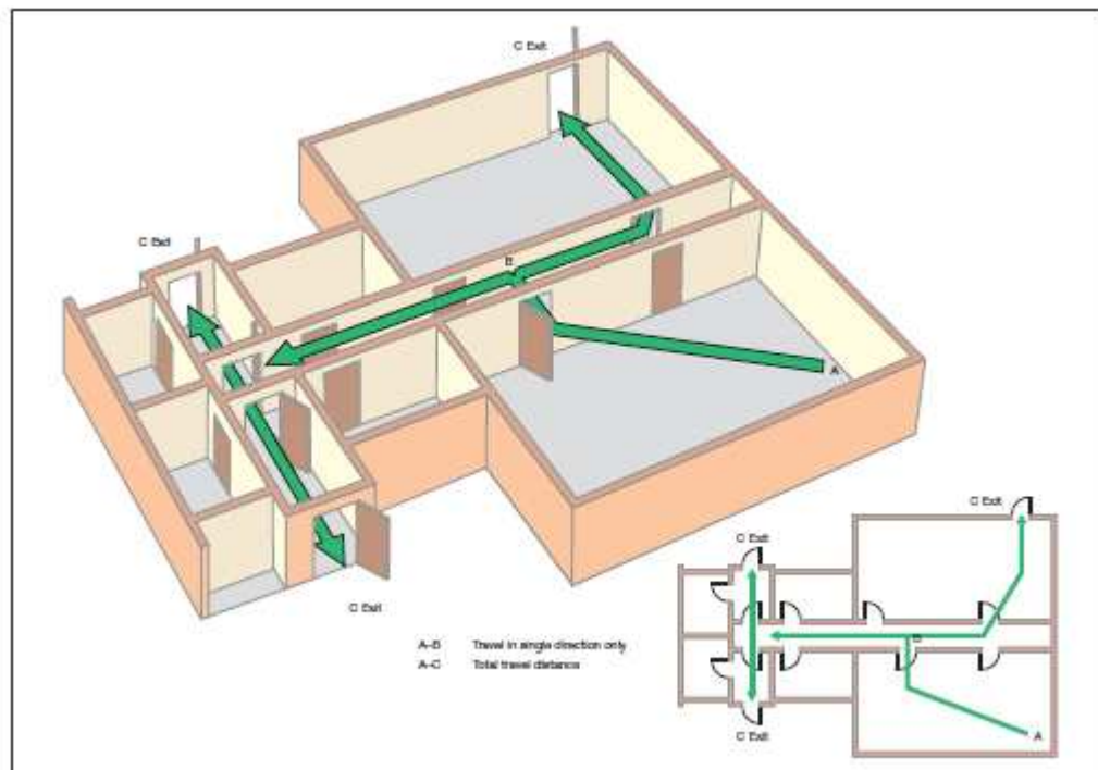
Figure 32: Dead end condition provided with an alternative exit (non sleeping areas)
