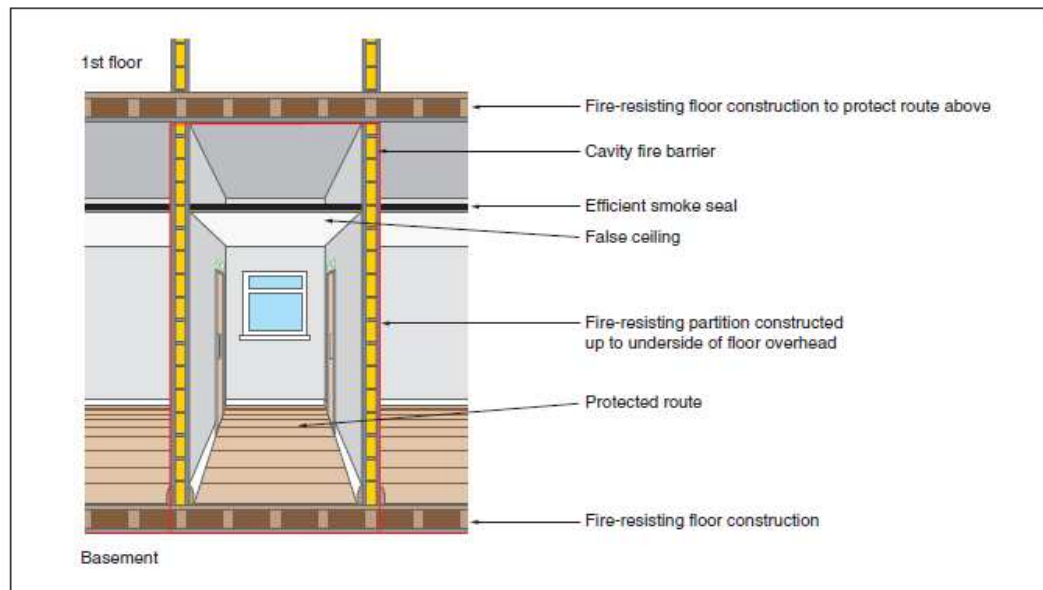
Figure 59: Fire-resisting construction
