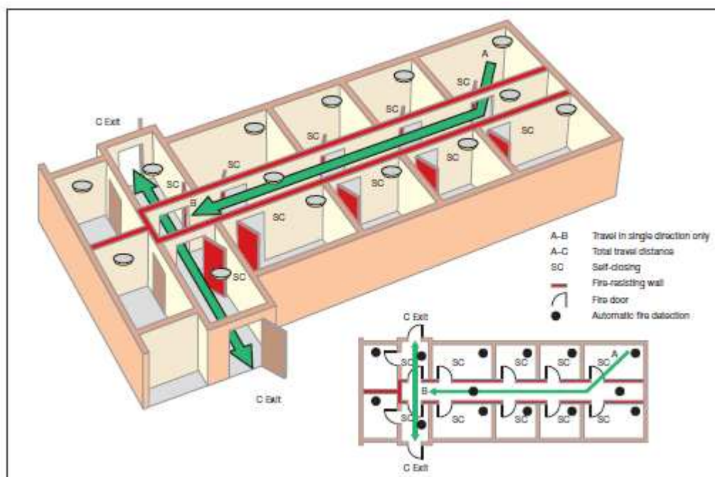
Figure 33: Dead end with fire resisting construction and automatic fire detection (in sleeping areas)
