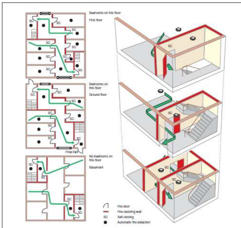
Figure 47: Three-storey (basement, ground and first floor)
