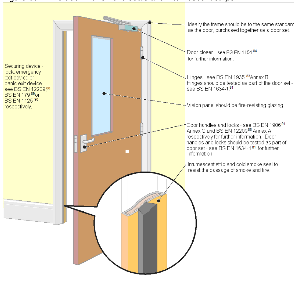
Figure 60: A fire door with smoke seals and intumescent strips
