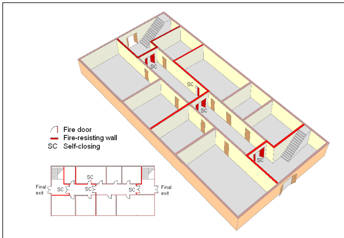
Figure 40: Separation of protected stairway
